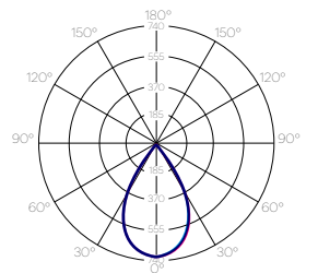
light distribution DOWN
