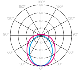
light distribution JET OUT
