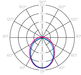
light distribution MID JET
